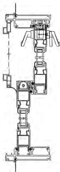
Fiberglass Sliding Patio Door, top view
