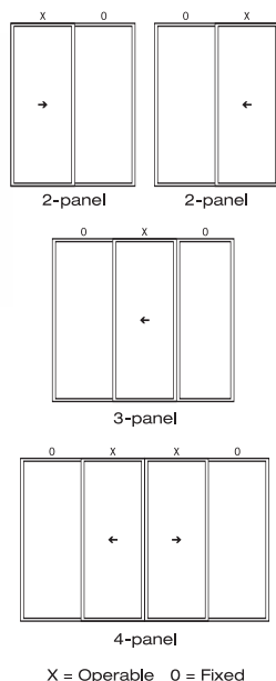
Fiberglass Sliding Patio Door configurations
