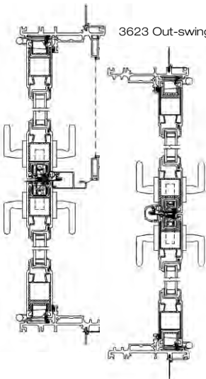
French Doors, In-swing and Out-swing top view
